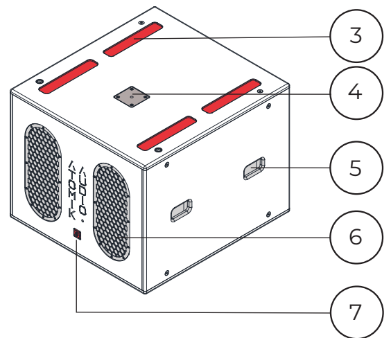
ISO VIEW
